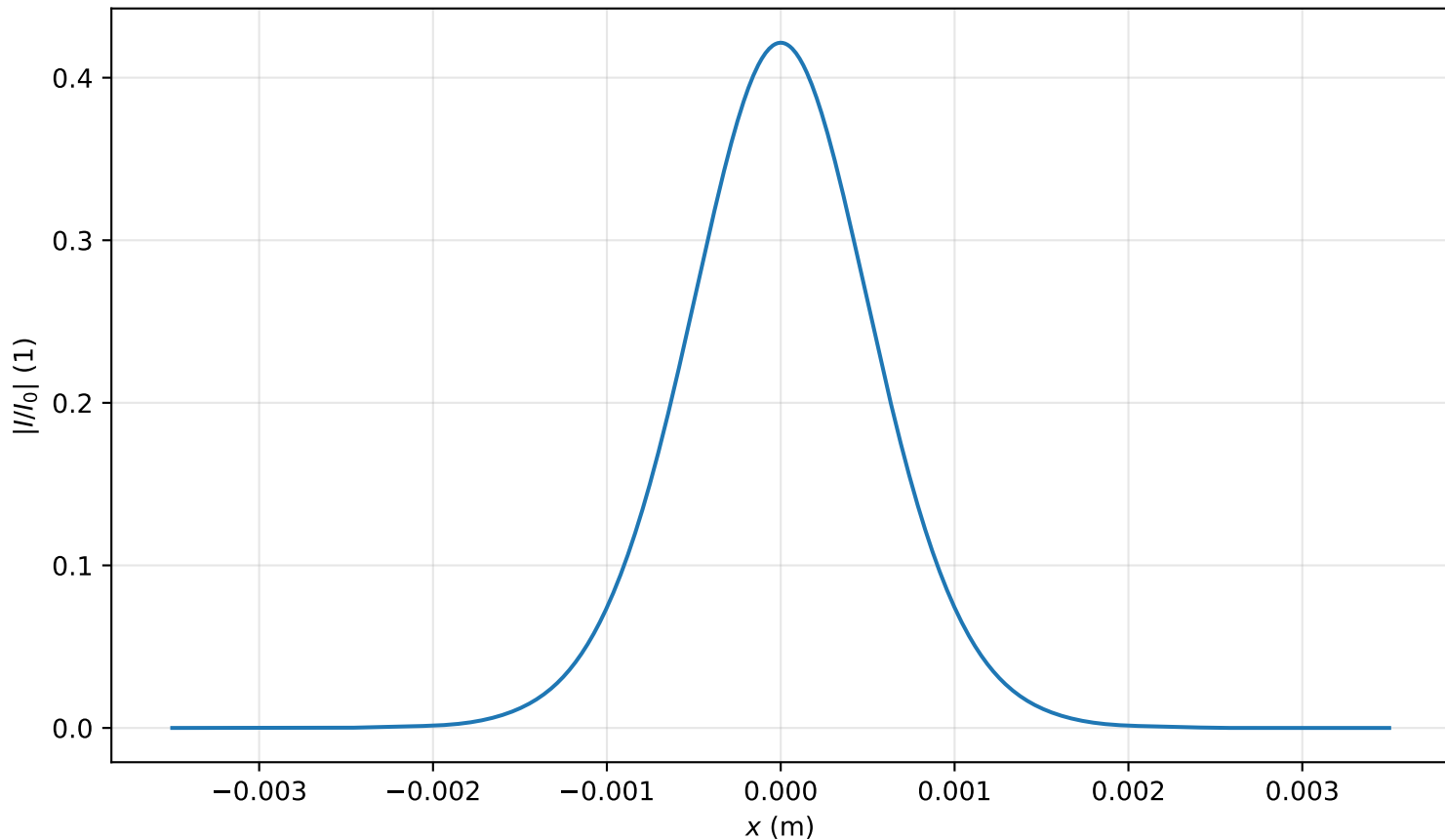
Intensity profile I(x, y = 0, z = 3.344m)/I_0 , P_{in}=0.4P_{cr} , artificial time
